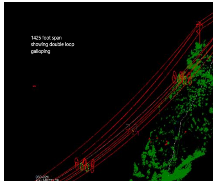
Figure 15: PLS CADD Showing Galloping
